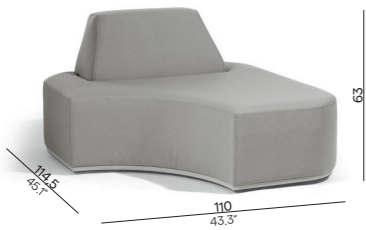
Left corner seat FUR0000331
